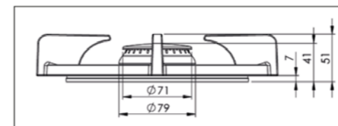
SMALL BURNER
